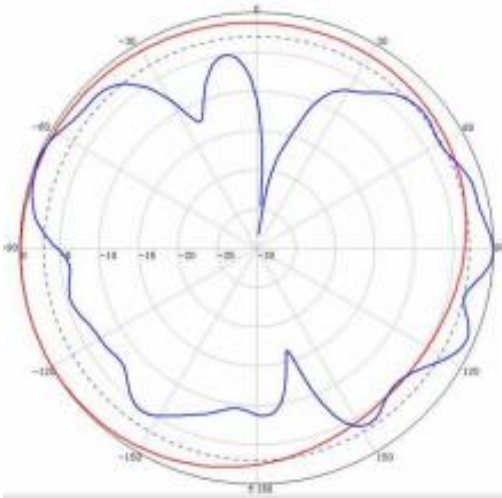
617~960MHz Typical pattern
