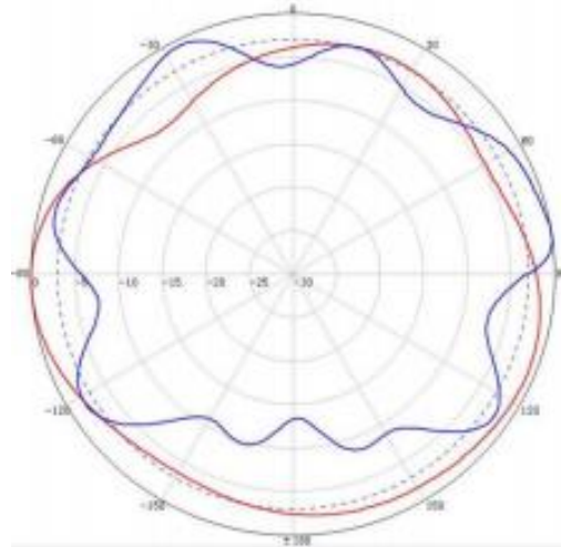
1710~2700MHz Typical pattern
